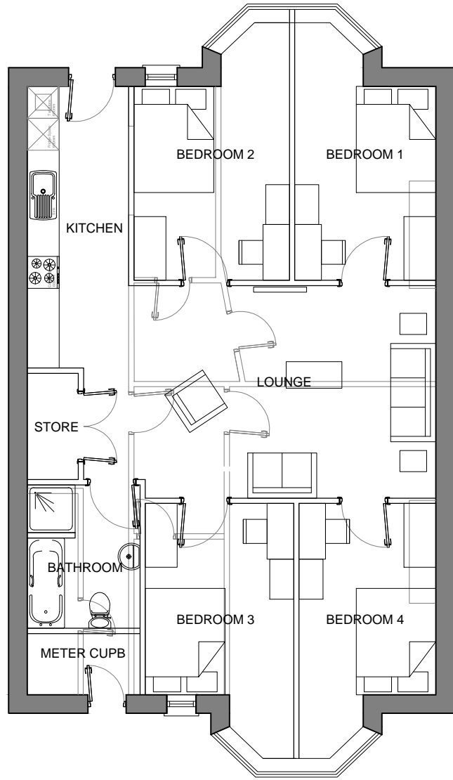
PROPOSED LOWER GROUND FLOOR PLAN SCALE 1:100
