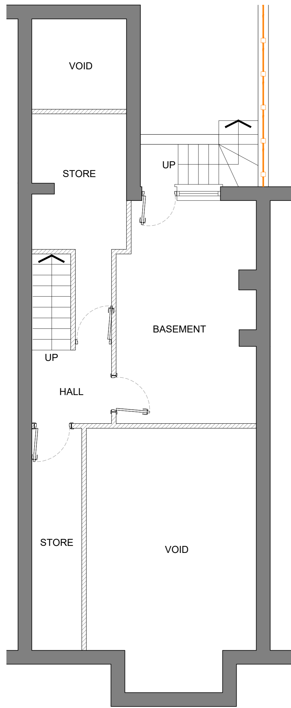
LOWER GROUND FLOOR PLAN
