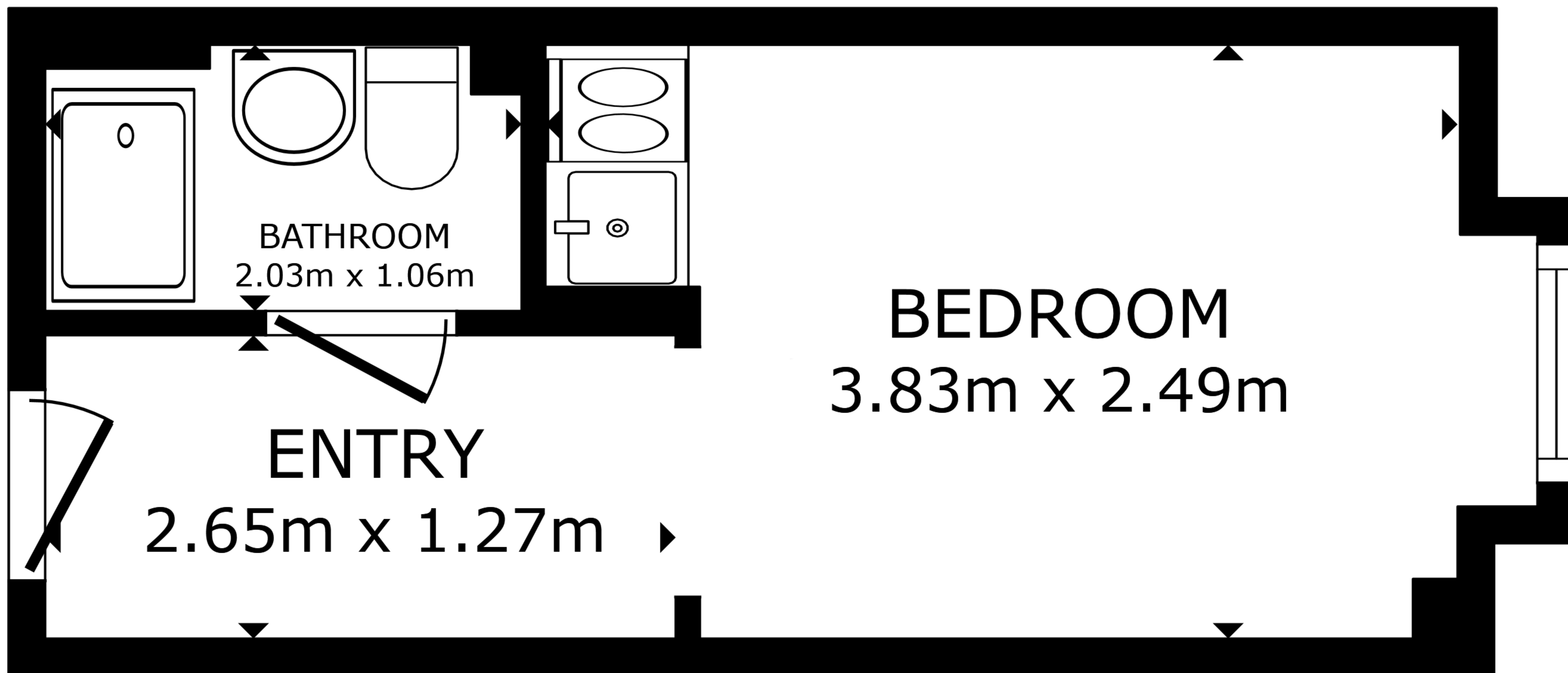
FLOOR PLAN
